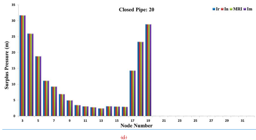
Figure 6. Surplus pressure of Hanoi network nodes for solutions of maximum reliability criteria when pipes No. (a) 4, (b) 5, (c) 6 and (d) 20 are lost due to failure
