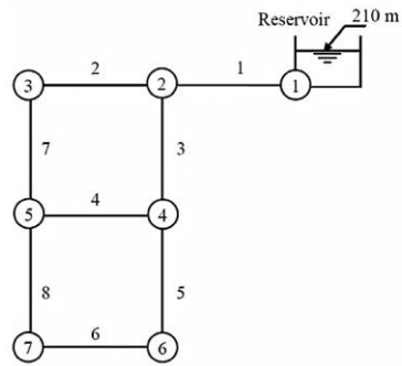
Fig.1 The layout of Two-loop network.
