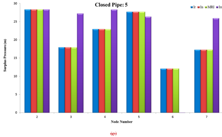
Fig. 43 Surplus pressure of nodes in two loop network for solution with maximum reliability criteria under failure of pipes No. (a) 2, (b) 3 and (c) 5
