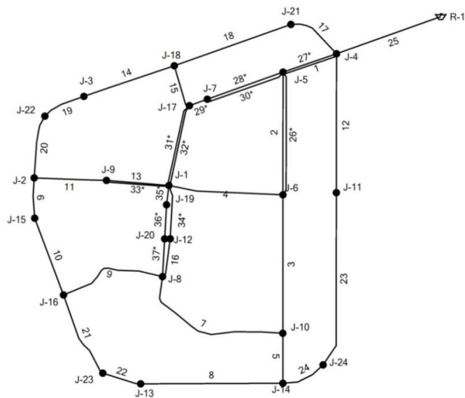
Fig. 9-7. Layout of Real-life network
