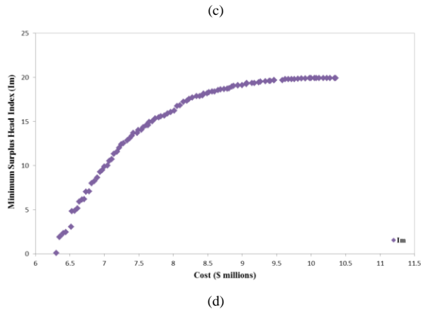
Fig-7-53. Pareto front of two-objective function optimization of the Hanoi network, (a) Cost- I_r-I_{r2} , (b) Cost-
