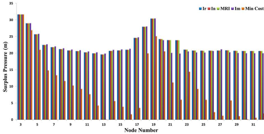
Fig-7-54. Nodal surplus pressure of Hanoi network for solutions of maximum reliability criteria and minimum cost
