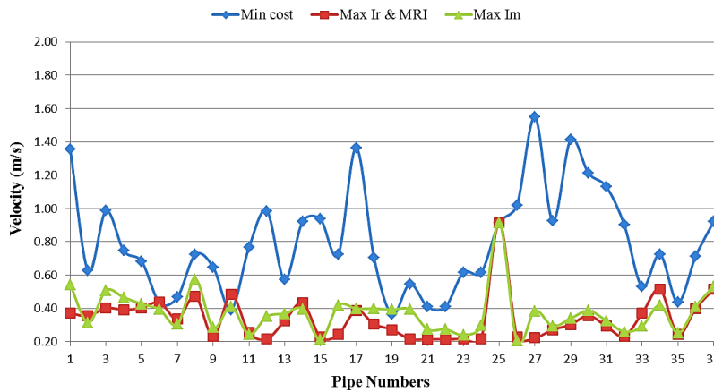
Fig. 13-17. Velocity variations in pipes for the solutions of minimum cost and maximum I_r , MRI and I_m criteria
