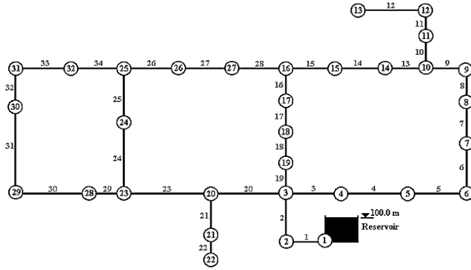
Fig. 5 Layout of Hanoi network
