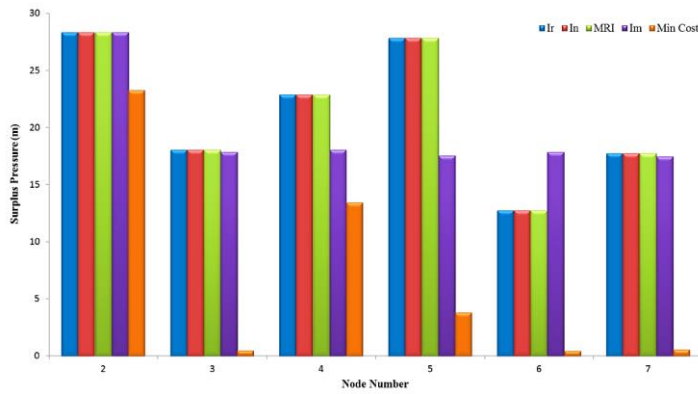
Fig-3.2. Surplus pressure of nodes in two-loop network for solutions of maximum reliability criteria and minimum cost
