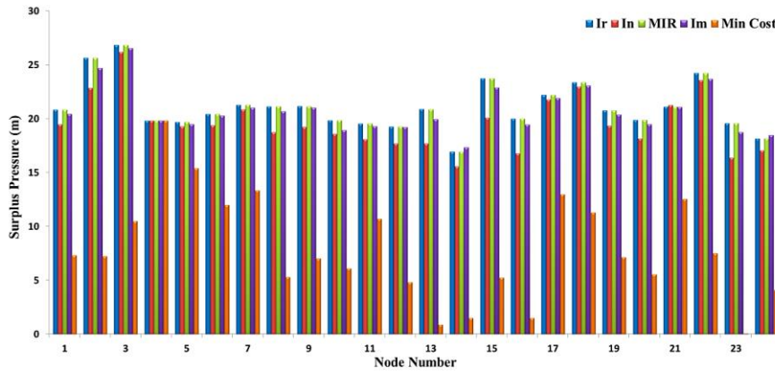
Fig-1196. Surplus pressure of the real- life for solutions of maximum reliability criteria and minimum cost
