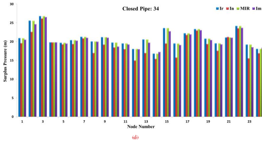
Fig. 12-10. Surplus pressure of nodes in Real-life network for solutions of maximum reliability criteria under failure of pipes No. (a) 18, (b) 21, (c) 27 and (d) 34
