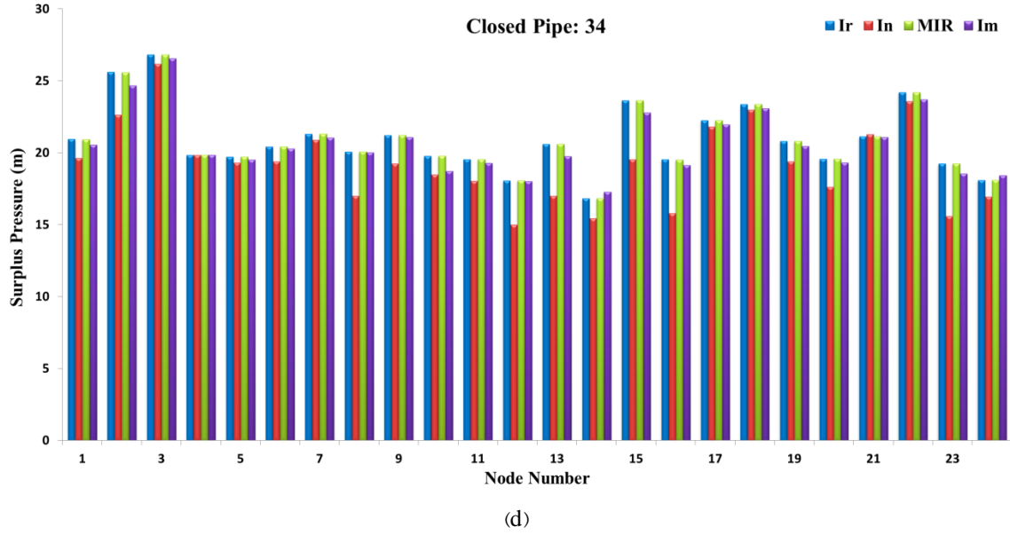
390 Fig 10. Surplus pressure of nodes in Real- life network for solutions of maximum reliability criteria under failure of pipes No. (a) 18, (b) 21, (c) 27 and (d) 34
