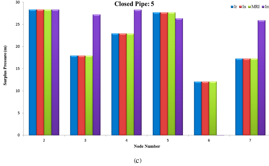
Fig. 3 Surplus pressure of nodes in two-loop network for solution with maximum reliability criteria under failure of pipes No. (a) 2, (b) 3 and (c) 5
