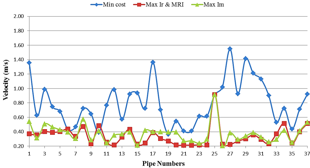
Fig 11. Velocity variations in pipes for the solutions of minimum cost and maximum I_r , MIR and I_m criteria
