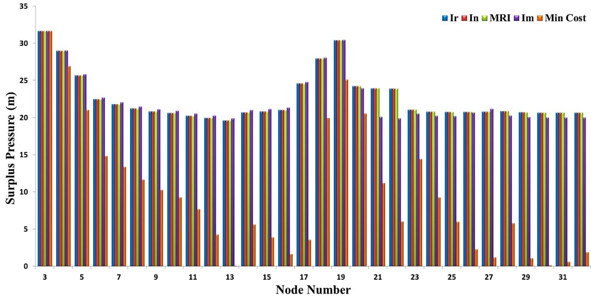
Fig 5. Nodal surplus pressure of Hanoi network for solutions of maximum reliability criteria and minimum cost Table 3 shows the statistical parameters for each pipe of Hanoi network due to different runs of single-objective optimizations by GANetXL. According to this table, Pipes No. 4, 5, 6 and 20 that have standard deviation and variation coefficient equal to zero have been chosen for reliability evaluation when there is a failure in the network.
