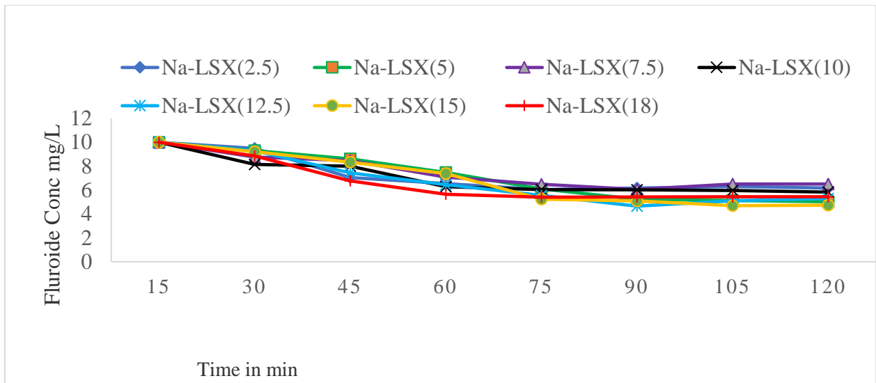
Figure 3: Fluoride removal using Na-LSX modified zeolite with different dosage of HDTMA (Model water composition: (F^-) i = 10 \text{ mg/L} , Blank = 10 \text{ mg } F^-/\text{L} without adsorbent)
