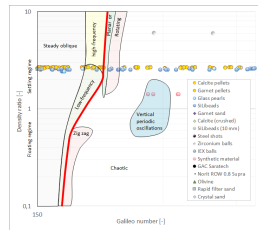
Figure 10 Path trajectory regime plot according (Zhou and Dušek, 2015; Raaghav, 2019) (zoomed area). The chaotic regime applies to the right of the red line
