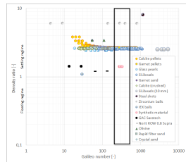
Figure 9 State diagram, Galileo number Ga versus specific gravity number \tilde{\beta} with examined particles
