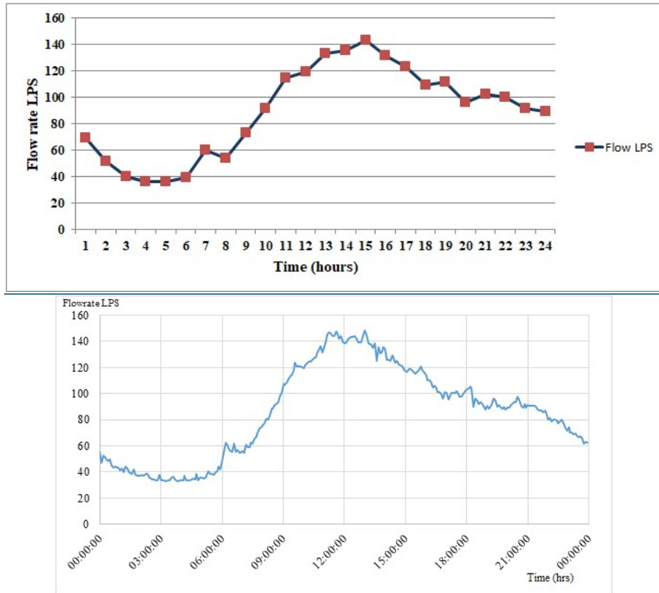
Figure 2 Daily average water demand of the study area.
