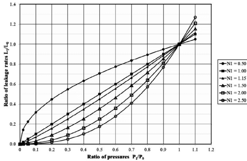
Figure 4 Relationships between pressure and leakage rate using the N1 Approach (Rozental, 2010)
