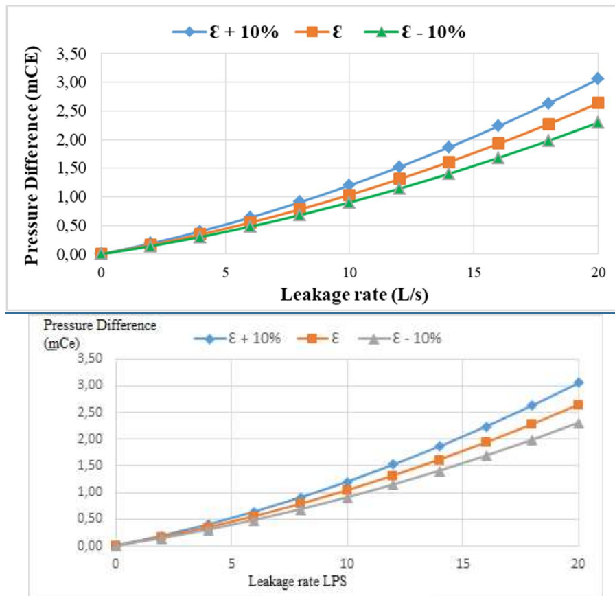
Figure 6-5 Influence of the error on the roughness of the pipe
