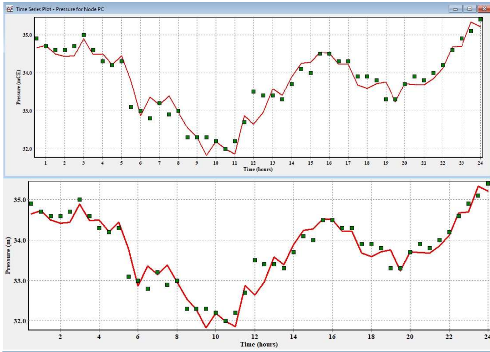
355 Figure 16-14 Pressure profile at PC
