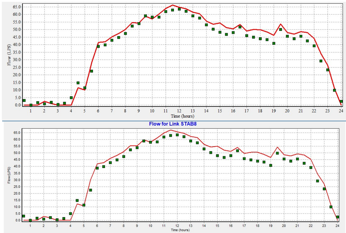
Figure 17-15 flowrate calibration
