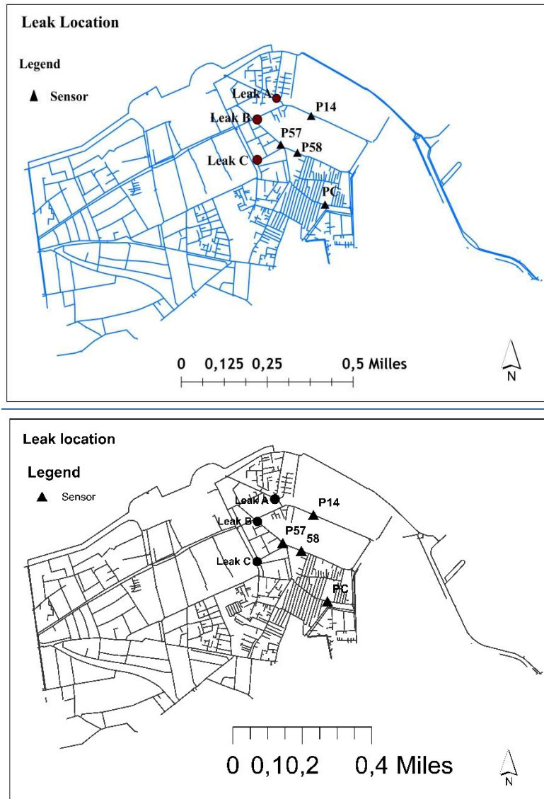
Figure 13-11 Sensors and leaks locations
