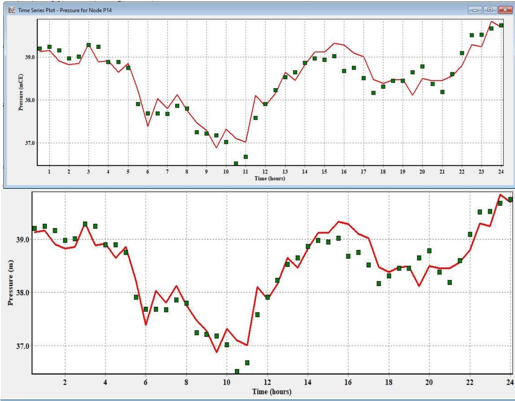
Figure 45-13 Pressure profile at P14
