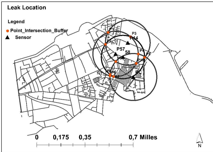
Figure 18-16 The spatial intersection of circles
