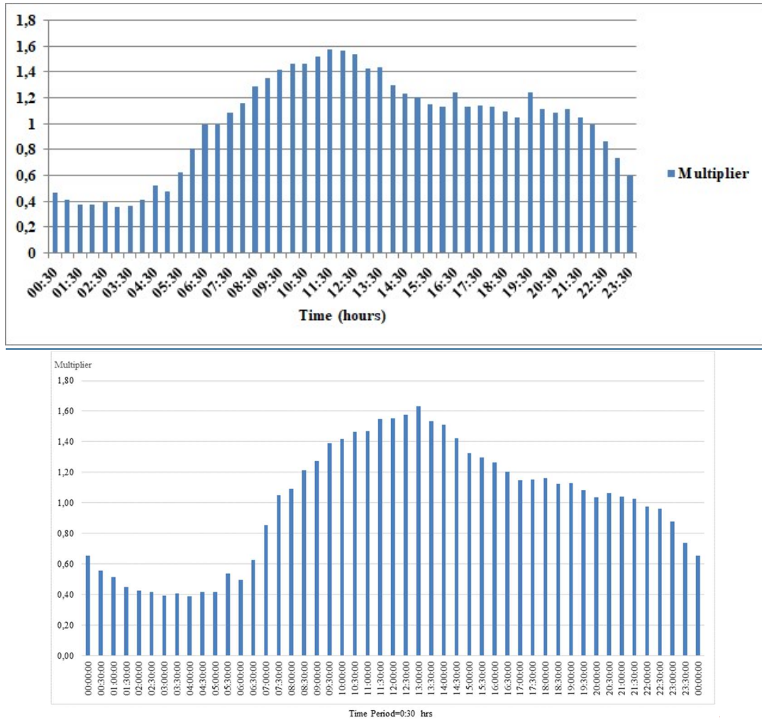
145 Figure 5-4 daily consumption patterns in the study area
