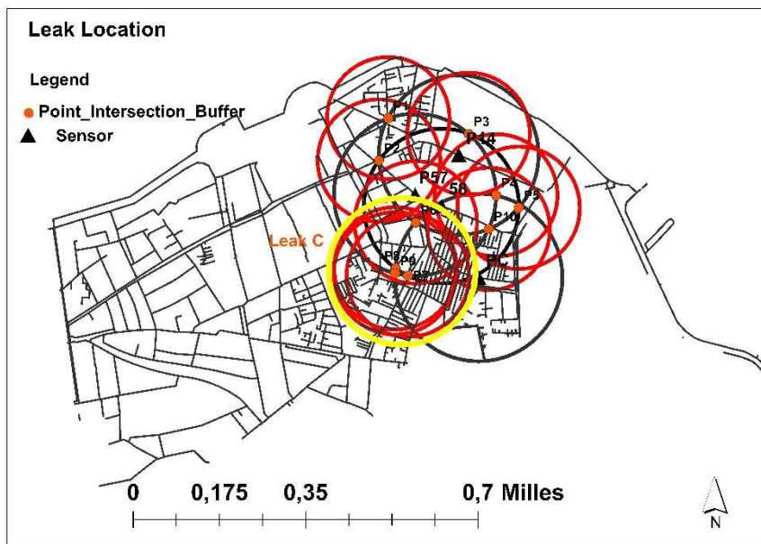
Figure 19-17 Spatial location of the leak LC
