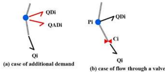
Figure 7-7 Ways to model a water leak in a hydraulic network model ( Sebbagh et al., (2018) )
