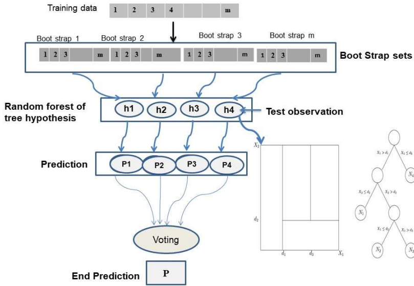
Figure 11 Random Forest Tree
