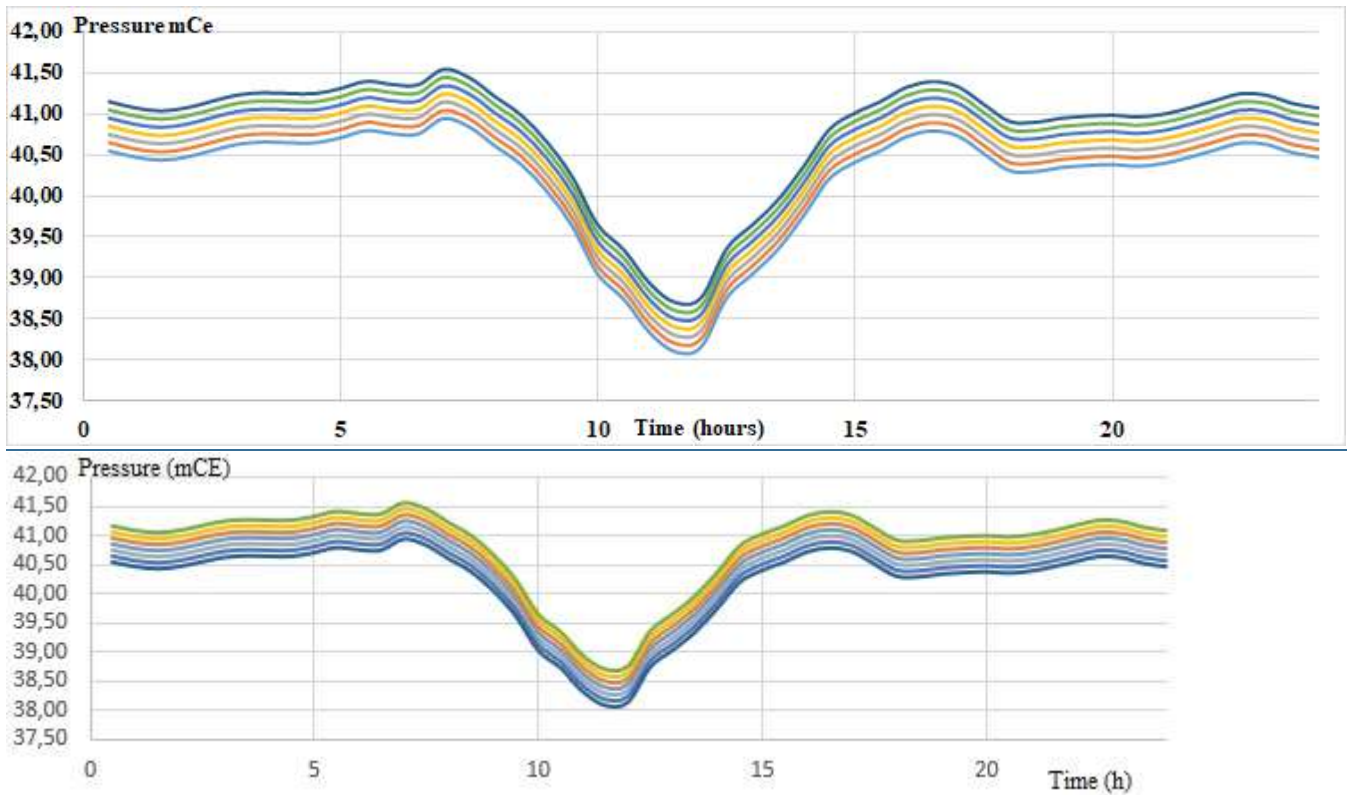
Figure 12-10 The reference pressures profile at P14
