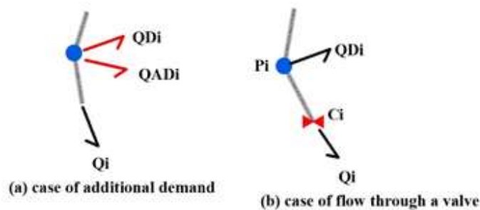
Figure 2 Ways to model a water leak in a hydraulic network model
