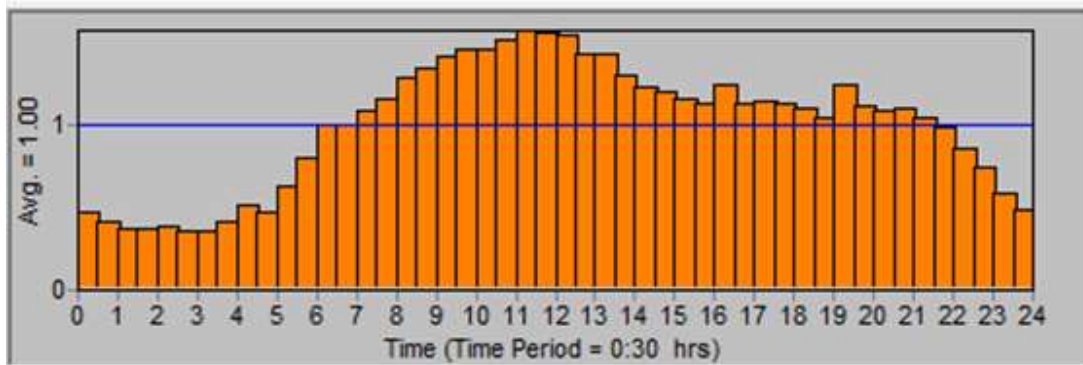
Figure 1 daily consumption patterns in the study area
