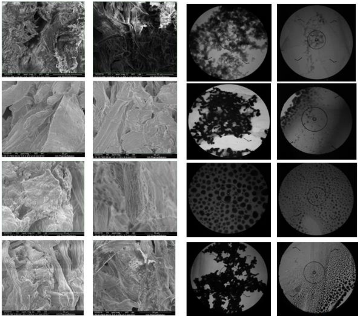
Figure 2: (a) Images obtained from SEM using 2:1 NaBH 4 /AgNO 3 ratio. (b) Images obtained from SEM using 10:1 NaBH 4 /AgNO 3 ratio. (c) TEM images using 2:1 NaBH 4 /AgNO 3 ratio. (d) TEM images using 10:1 NaBH 4 /AgNO 3 ratio
