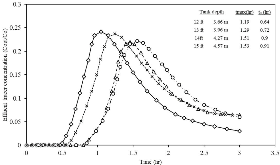
Fig 5. Effluent concentration with a baffle height of 1.52 m in tank depth variations.
