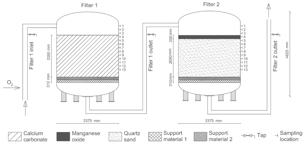
Figure 1: Initial design of a production line at Truelshjerg waterworks (revised from Søborg et al. 2015).
