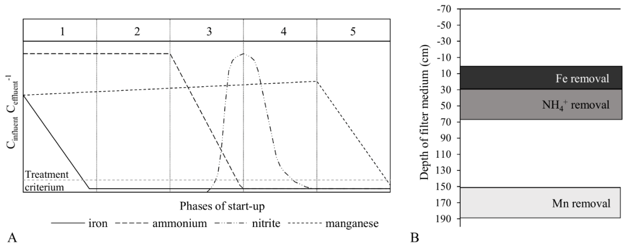
Figure 9: A. Conceptual phases of the start-up period in drinking water biofilters (modified from Frischherz et al. 1985). B.
