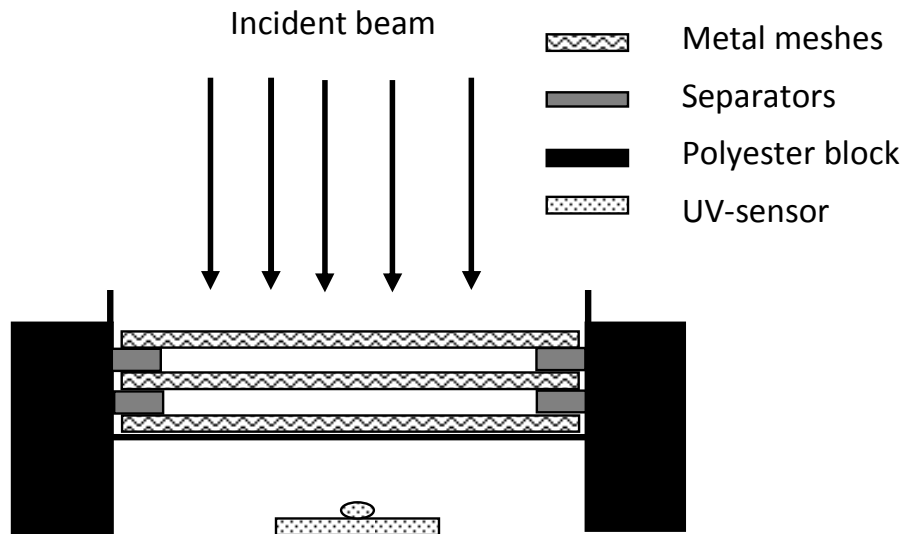
Fig. 2. Schematic view of the experimental setup for light distribution measurements.
