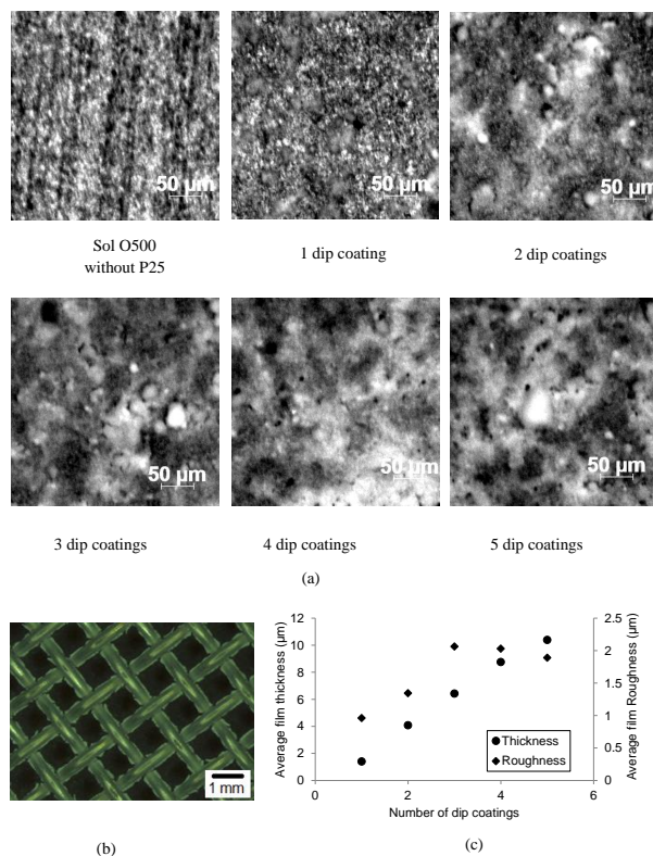
Fig. 6. (a) Microscopic images of coating films showing increasing of \text{TiO}_2 agglomerates by increasing of number of dip coatings. (b) Microscopic image for woven mesh coated by three dip coatings on O500-P25 sol gel and dried at final temperature 300 °C. (c) Average surface thickness and roughness of O500-P25 \text{TiO}_2 film over stainless steel flat plate with different number of dip coatings at 300 °C measured by Veeco Dektak 8 Stylus Profiler.
