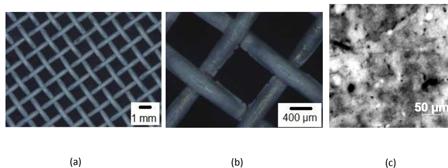
Fig. 7. Microscopic image of the stainless steel woven mesh coated with EPD method using O-500 sol gel modified with \text{TiO}_2 suspension: (a) low magnification; (b) high magnification; (c) microscopic image of coating film with O500-P25 sol gel by EPD using DC current (6 V, 2.5 A) during 1 min deposition time.
