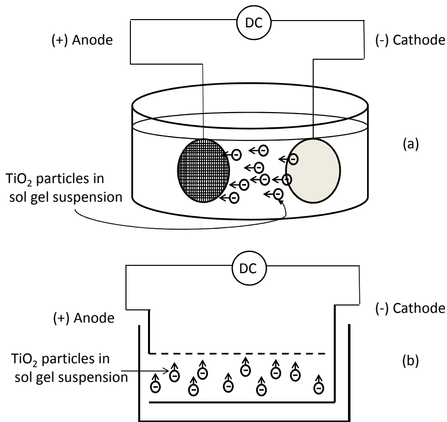
Fig. 1. Schematic view of electro-deposition cell. (a) A vertical coating setup for the small mesh discs. (b) A horizontal coating setup for the large-scale meshes.
