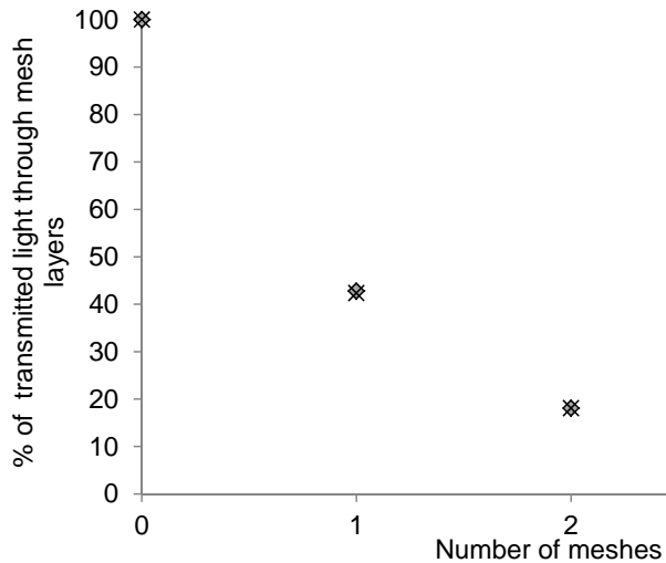
Fig. 10. Light transmission through coated woven meshes ( r = 0.45 ) in a non-absorbing medium (distilled water). Measured intensities: (◆) 0.2 cm mesh separation; (x) 1 cm mesh separation.
