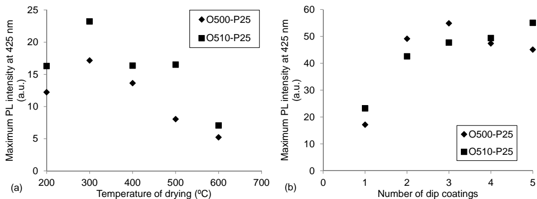
Fig. 5. Maximum PL intensity at 425 nm for woven meshes coated with O500-P25 and O510-P25 sol solutions as a function of (a) final drying temperature (one dip coating) and (b) number of dip coatings (final drying at T = 300\text{ }^{\circ}\text{C} ).
