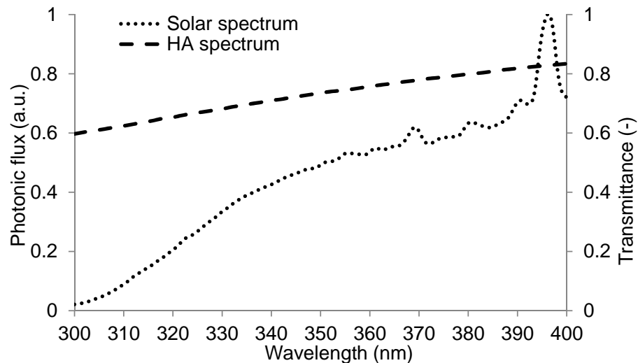
Fig. 3. Transmission spectrum of HA was measured by Hach Lange DR 5000 spectrophotometer and the normalized emission spectrum of artificial solar light was measured by Black C-50 spectrometer, a product of StellarNet Inc.
