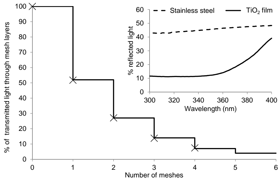
Fig. 9. Light transmission through uncoated woven meshes (for which r = 0.48 ) in a nonabsorbing medium (distilled water). The solid line represents model calculations according to Eq. (1); (x) measured intensities with 1 cm mesh separation. Inset: reflection of stainless steel flat plate and TiO 2 film measured with the integrated sphere spectrometer.
