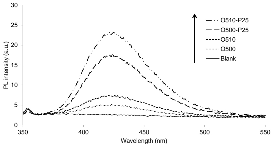
Fig. 4. PL spectra of 2-OHTA formed by 45 min irradiation of different coated meshes. Initial TA concentration is 5 \times 10^{-4} M; excitation is at 315 nm; final drying temperature is 300 °C.
