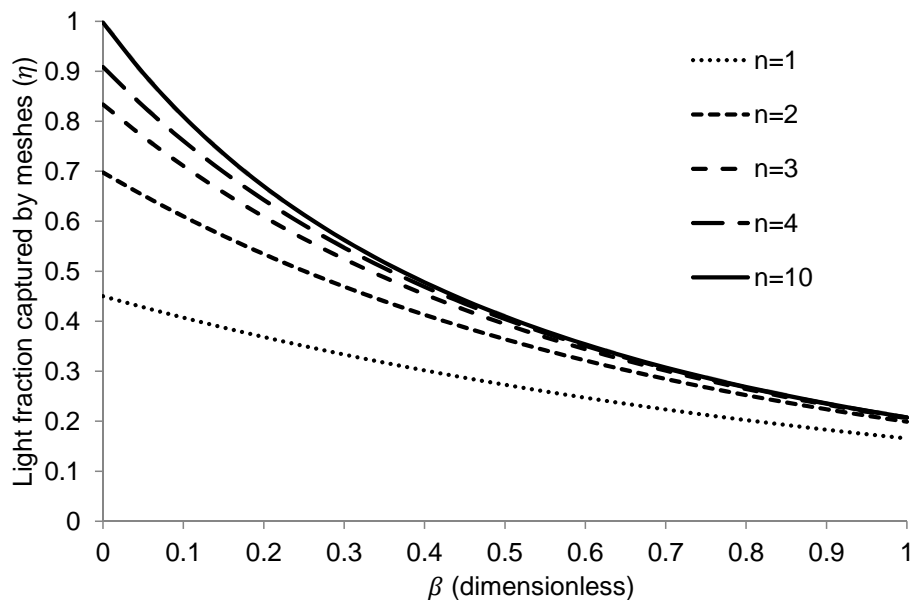
Fig. 12. The fraction of captured light by the coated meshes ( r = 0.45 ) as a function of the dimensionless \beta parameter in a light absorbing medium.
