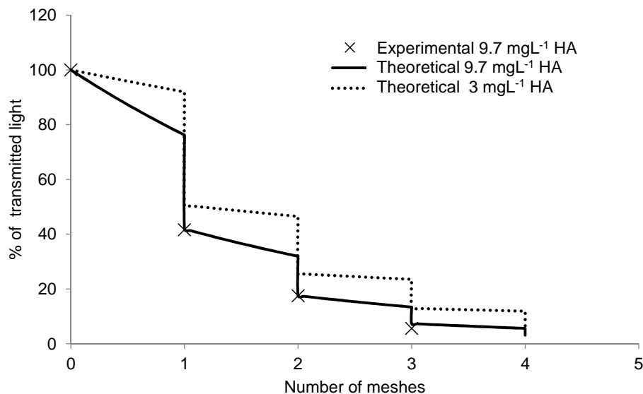
Fig. 11. Experimental measurements and theoretical calculations for the percentage of the transmitted UV solar light (300–400 nm) through coated woven meshes ( r = 0.45 ) with separation distance 1 cm in the presence of different concentrations of HA.
