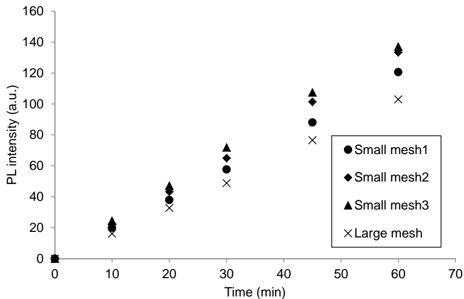
Fig. 8. Maximum PL intensity at 425 nm as a function of time for three single woven disc meshes and single woven sheet (19 cm × 32 cm), coated by EPD, after corrections for area-to-volume ratio.
