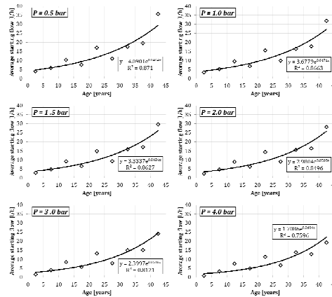
Figure 7. Relationship between average starting flow and meter age for the six different test pressures.
