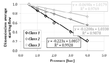
Figure 8. Relationship between average starting flow and test pressure for the different meter age classes.
