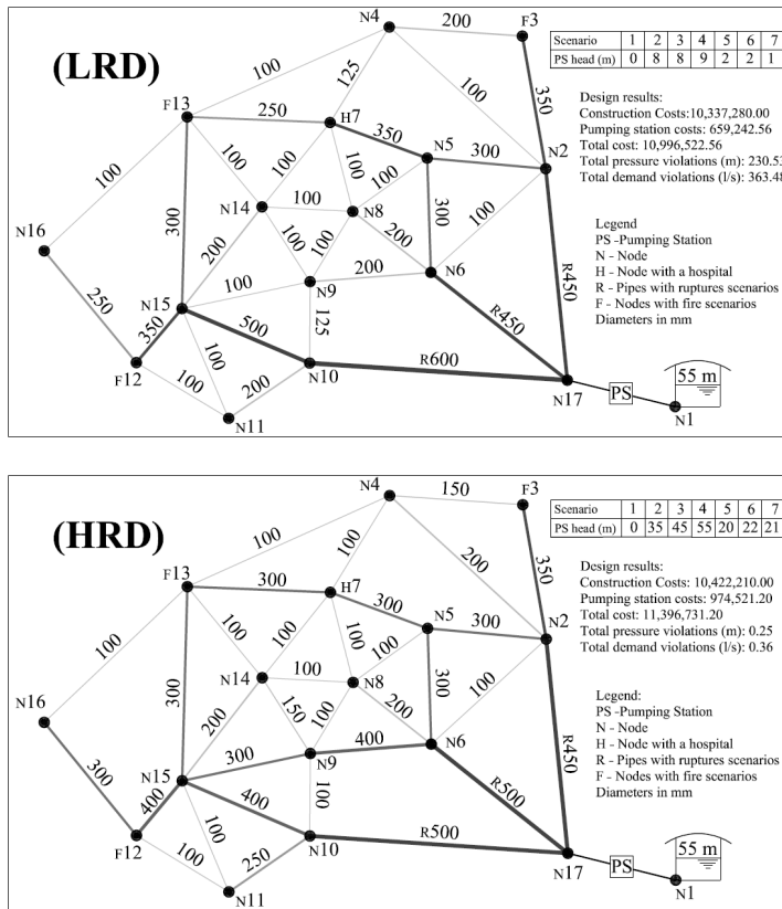
Fig. 3. Designs for case study 2: (LRD) low robustness and (HRD) high robustness.
