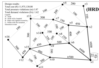
Fig. 2. Designs for case study 1: (PDD) peak discharge (LRD) low robustness and (HRD) high robustness.
