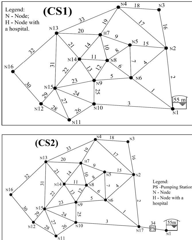
Fig. 1. Network schemes: case study 1 (CS1) and case study 2 (CS2).
