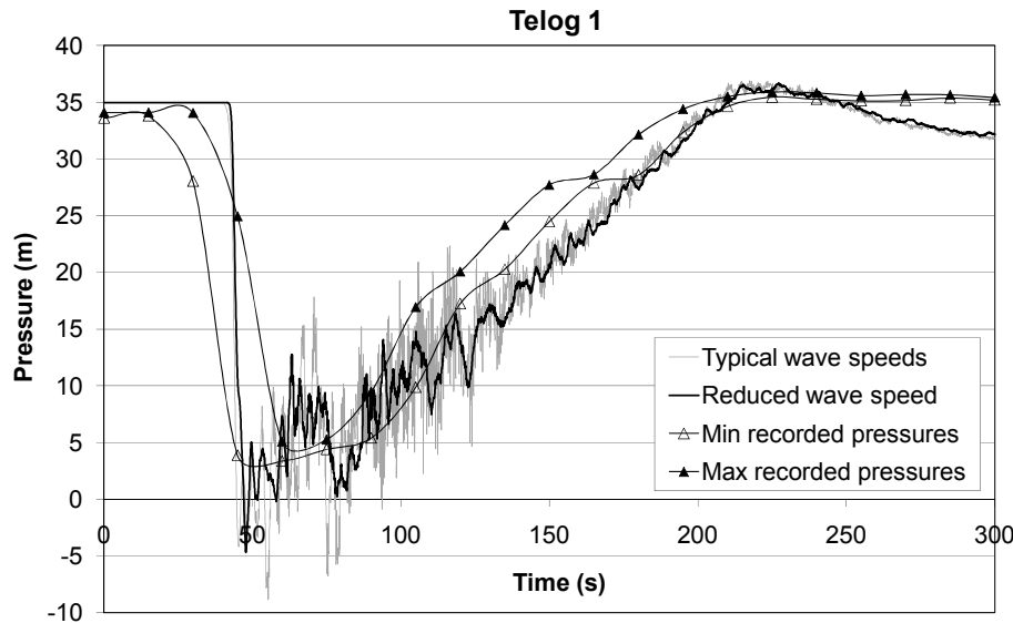
Fig. 2. Comparison of pressures recorded at one distribution system site with pressures modelled with typical wave speeds and with a reduced wave velocity in cast-iron pipes (four pressure values per second were measured by the pressure recorders but only the minimum and maximum pressures over 15 s intervals were saved ( \Delta \blacktriangle )).
