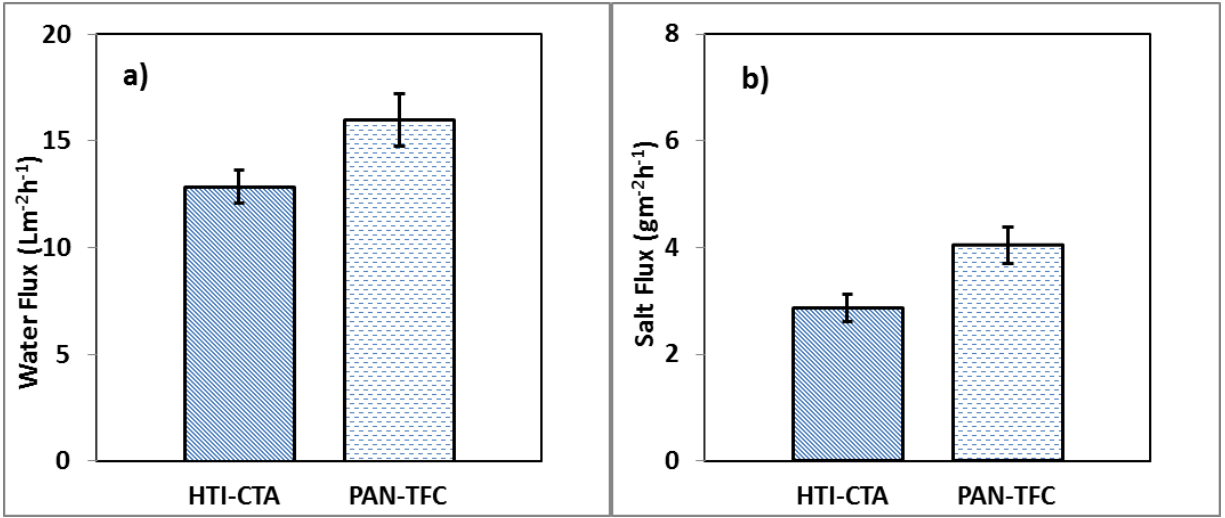
Figure 9 Forward osmosis water flux and salt flux for the PAN-TFC membrane. Experimental conditions: feed solution: DI water, draw solution: 1 M NaCl, FO mode, volumetric flow-rate of feed and draw 0.6 L/min, temp 25° C, zero transmembrane pressure. Results are an average of three experiments with different coupons. Error bars indicate standard
