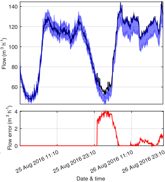
(b) Water flow q_{12} in pipe 12
