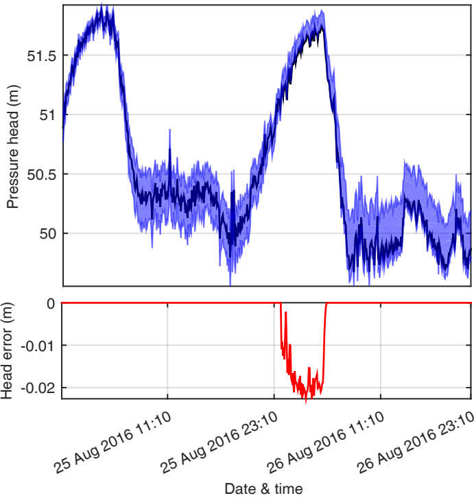
(a) Pressure head h_9 at node 9
