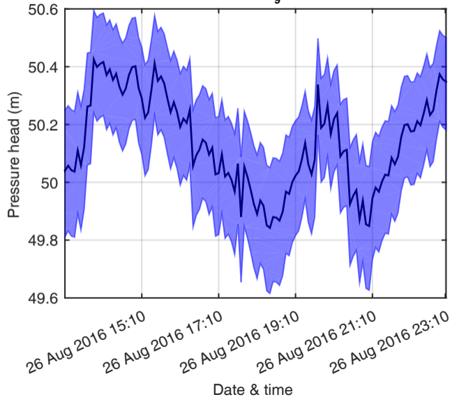
(b) Pressure head h_9 at node 9
