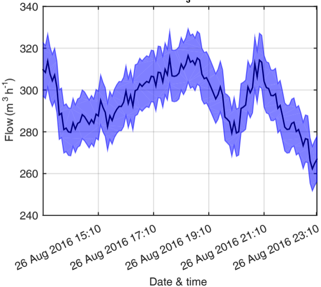
(a) Water flow q_3 in pipe 3
